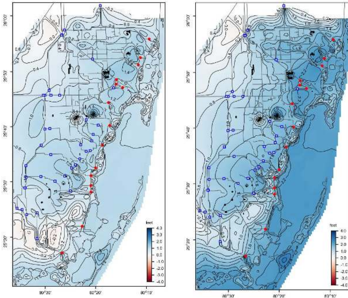
Figure 4. Difference in average wet season heads (ft) for LOW SLR (left panel) and HIGH SLR scenario (right panel)
