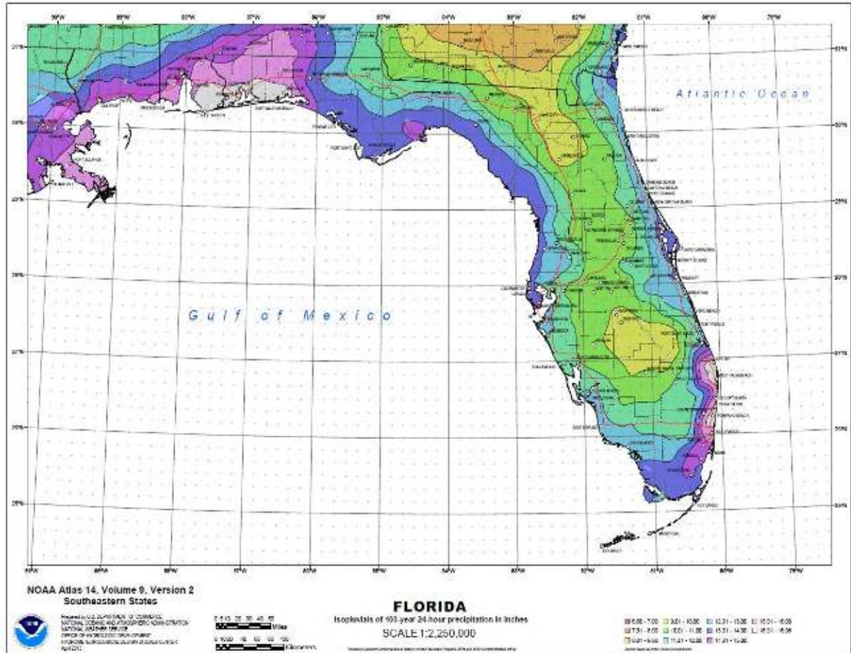
Figure 13. NOAA Atlas 14 map for daily, 100-year rainfall
