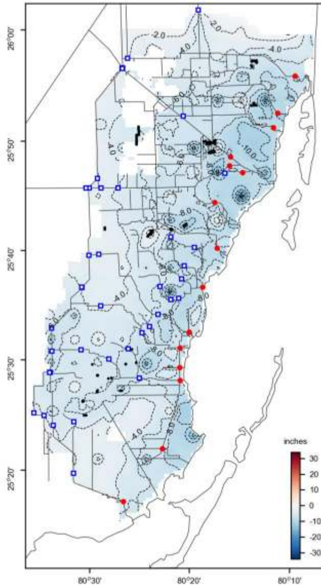
Figure 5. Decrease in soil storage above the water table for the high SLR Scenario
