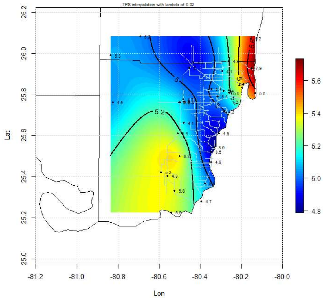
Figure 7. 1-in-100-year hourly rainfall totals (inches) based on thin-plate-spline (TPS) smoothing of station data (in black).
