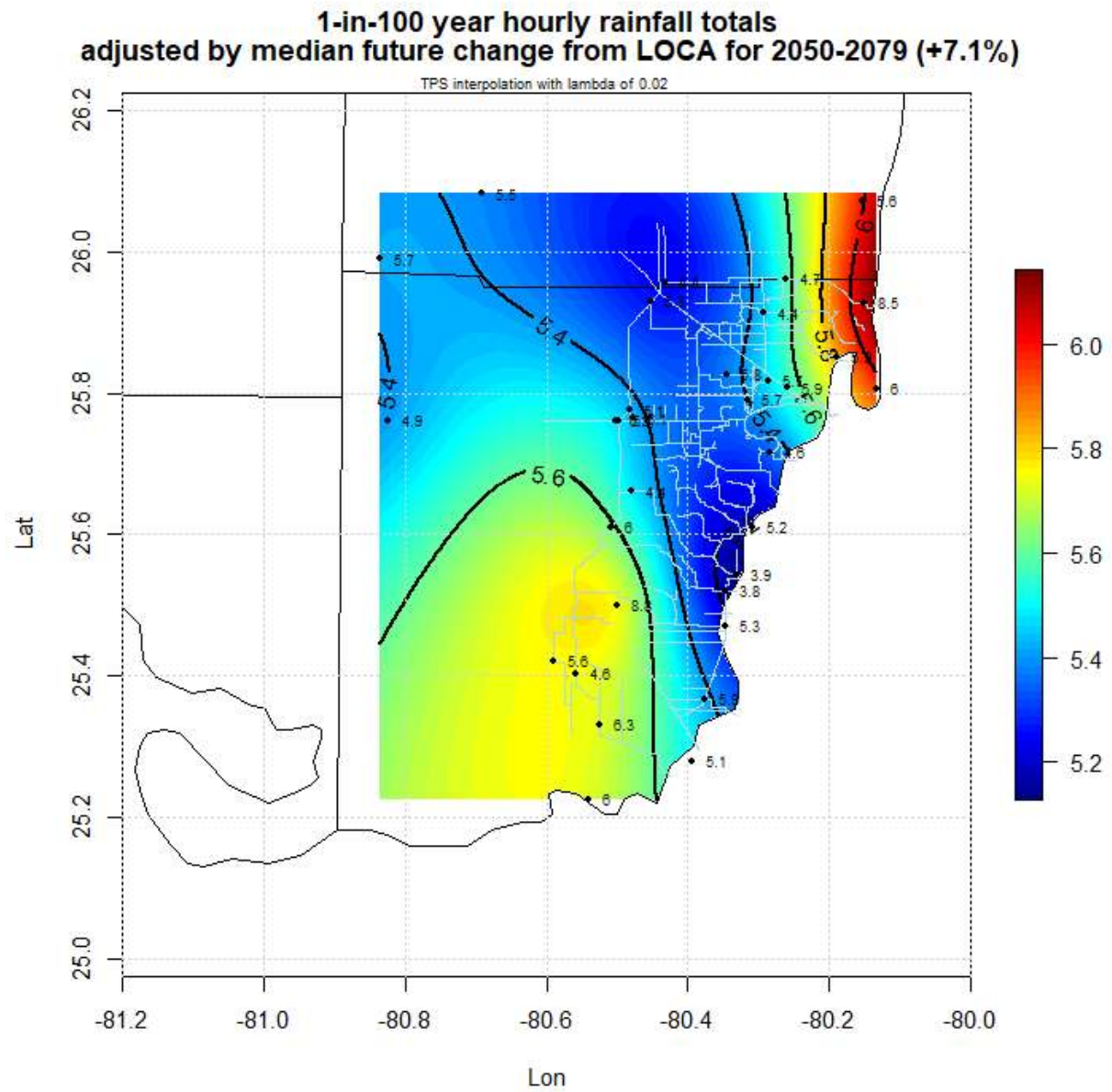
Figure 9. Estimated future 1-hour, 100-year rainfall predicted using LOCA rainfall.
