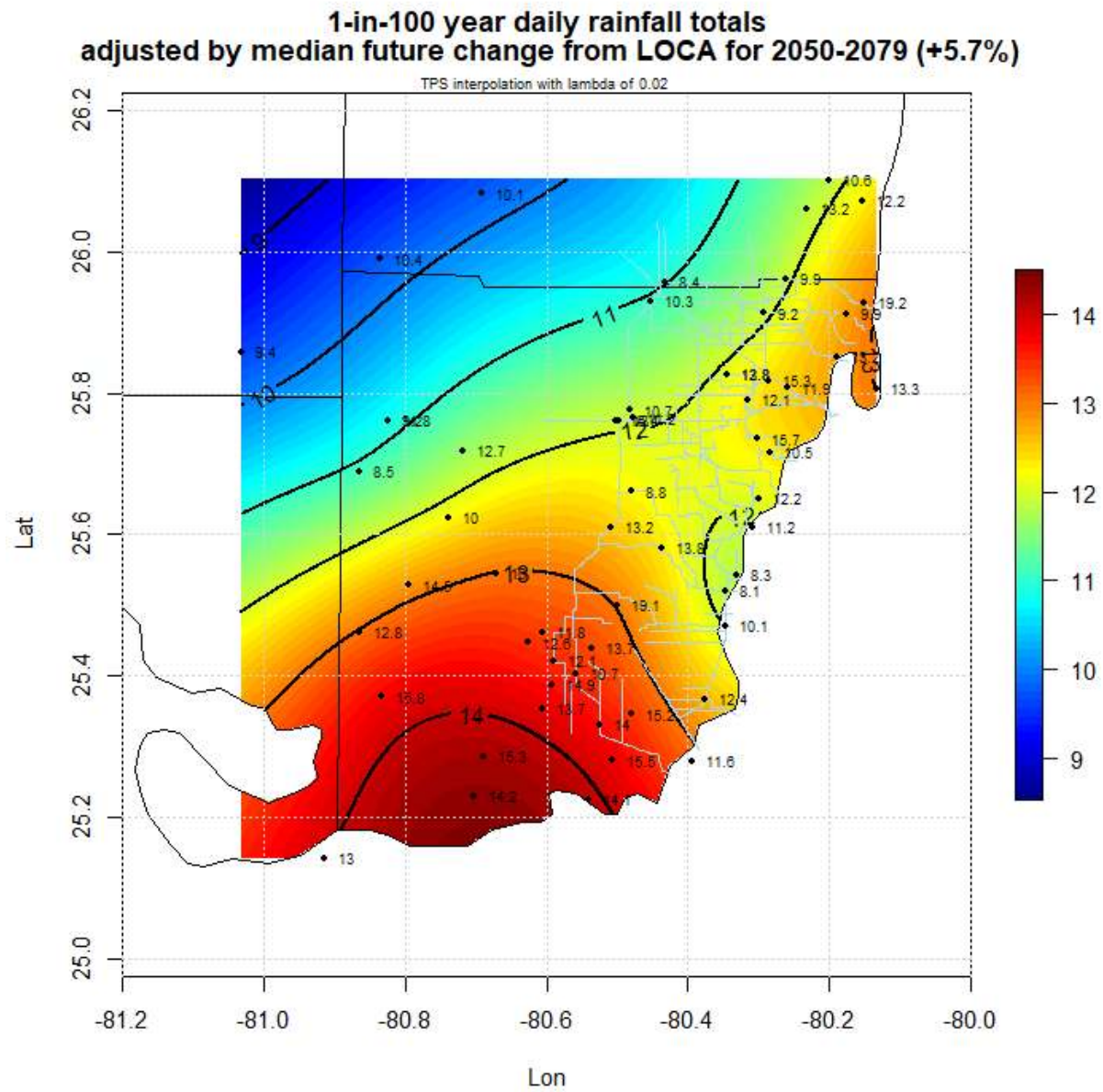
Figure 10. Estimated future daily rainfall predicting using LOCA data.
