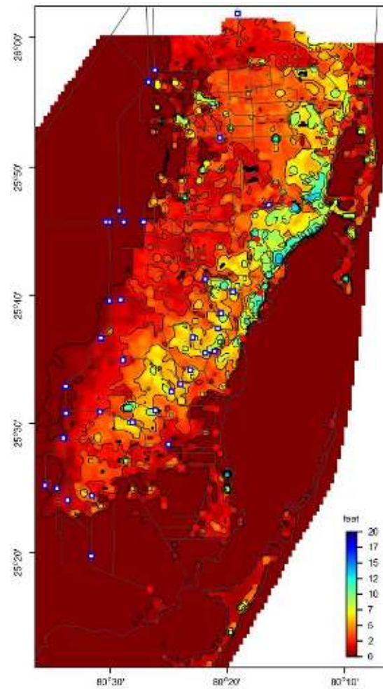
Figure 3. Average wet season heads (ft NAVD88) (left panel) and the average wet season depth to water table (ft) (right panel) for HIGH SLR + NO PUMPAGE sensitivity run.
